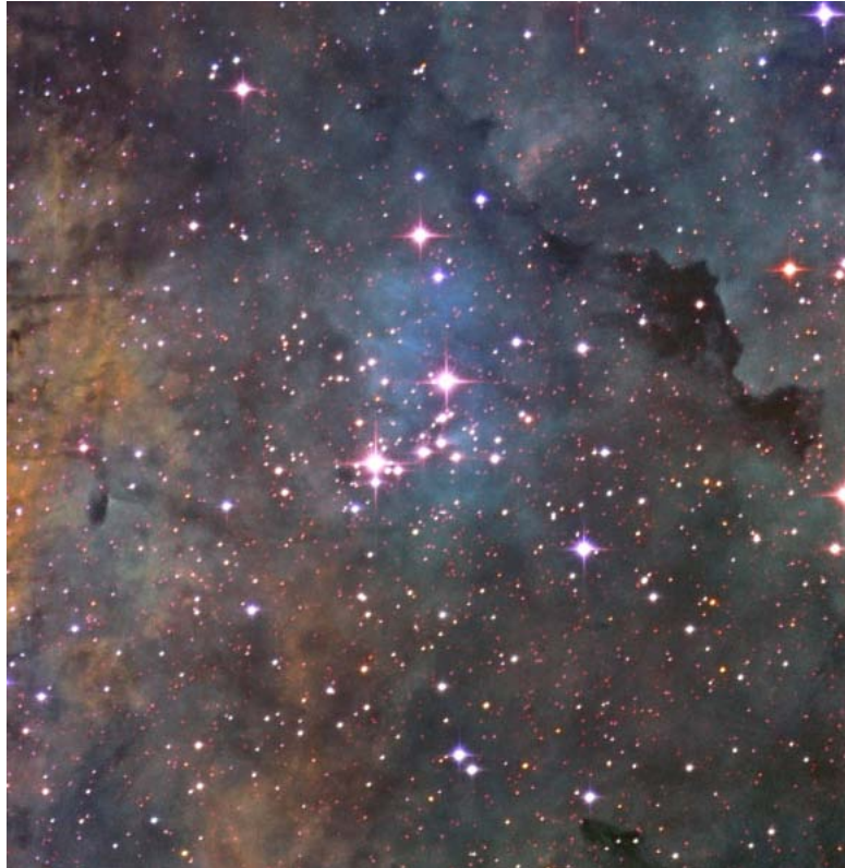
Figure 23. The young NGC 6910 cluster in the Cyg OB9 association. The figure is about 25 \times 25 arcmin. Image courtesy Johannes Schedler.
