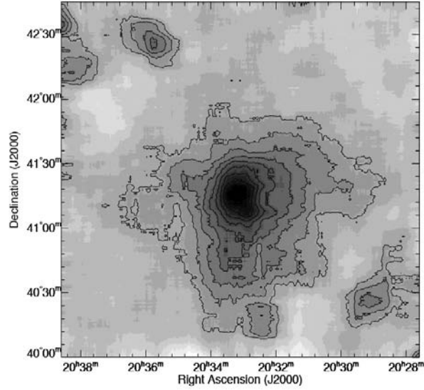
Figure 16. The stellar density distribution of the Cyg OB2 association derived from the 2MASS catalogue. Isodensity contours are in 10% steps of the peak density. From Knödlseider (2000).
