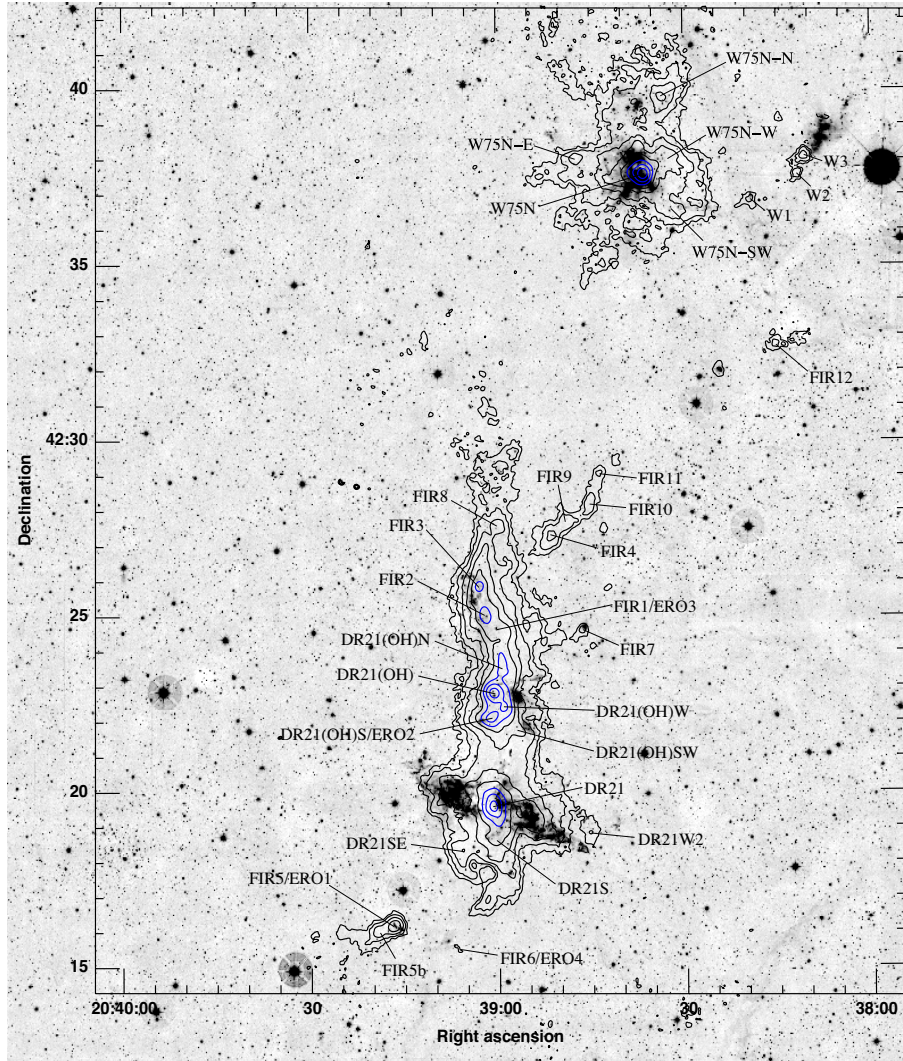
Figure 18. The DR 21/W75N complex. An \text{H}_2 image from the UKIRT WFCAM has superimposed contours of 850\ \mu\text{m} emission from SCUBA. A number of \text{H}_2 flows are seen emanating from the cold cores, in particular the major flow from DR 21. From Davis et al. (2007).
