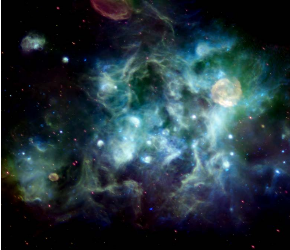
Figure 4. This image, created by Jayanne English (U. of Manitoba) and Russ Taylor (U. of Calgary), shows the Cygnus X region as a composite plot using data from the Canadian Galactic Plane Survey (CGPS) and the Infrared Astronomical Satellite (IRAS). The field covers approximately from Galactic longitude 76^\circ to 86^\circ and Galactic latitude -3.5^\circ to +5.5^\circ . The data have been colored such that synchrotron radiation appears as purplish-red (74 cm) and green (21 cm), and the IRAS bands in turquoise ( 60\ \mu\text{m} ) and 25\ \mu\text{m} (blue). The bright circular clouds at the upper right and lower left are the Gamma Cygni (G78.2+2.1) and G84.2-0.8 supernova remnants. Red point-like sources are background radio galaxies and quasars. Courtesy the Canadian Galactic Plane Survey.
