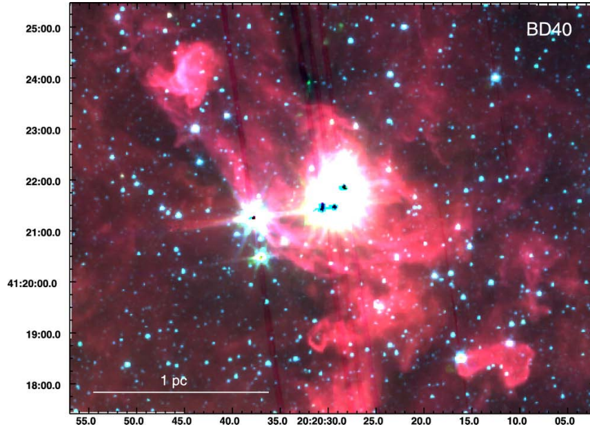
Figure 25. The region around the two Herbig Ae/Be stars BD +40°4124 and LkHα 224 = V1686 Cyg, as well as the peculiar binary LkHα 225 = V1318 Cyg as seen in a multi-band Spitzer image (3.6 \mu\text{m} is blue, 4.5 \mu\text{m} is green, and 8.0 \mu\text{m} is red). From Wang & Looney (2007).
