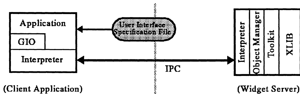
Figure 3. Widget Server Architecture
