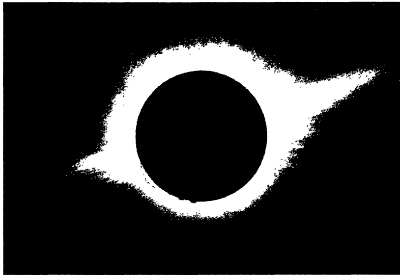
Figure 2. Illustration of the solar eclipse of November 30, 1853, from Moesta (1854a) (US Naval Observatory Library).
