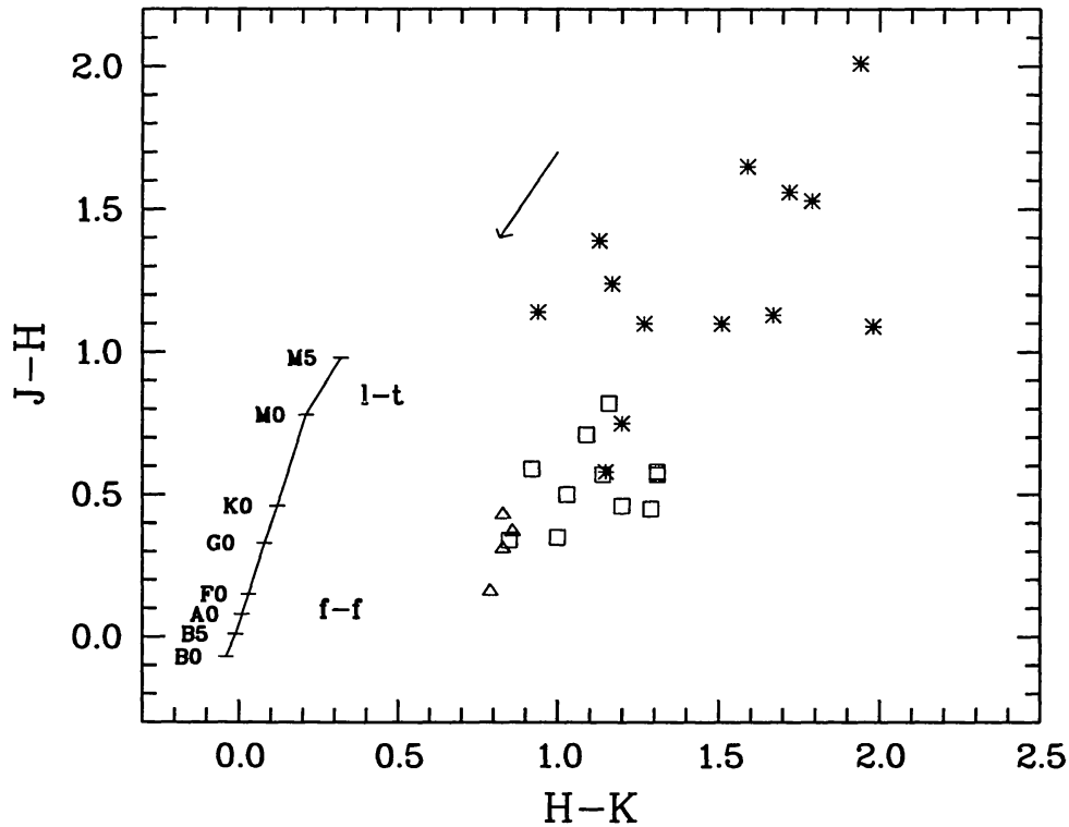
Figure 1. (J-H)-(H-K) diagram for B[e]-type stars. The different symbols denote B[e] stars in the Milky Way (asterisks), in the LMC (squares) and in the SMC (triangles). The location of stars with normal colours is indicated by the solid line. “f-f” denotes the approximate location of stars with IR excess due to f-f emission from stellar winds. “l-t” marks the area occupied by objects with late-type companions. The arrow gives the reddening line for A_V = 3 .
