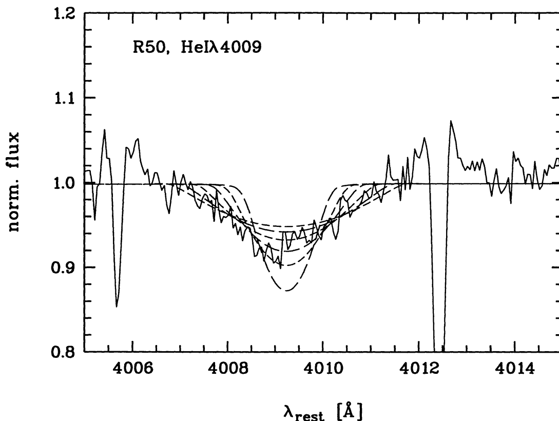
Figure 2. Section of the spectrum of R 50 in the SMC (spectral resolution \sim 20\,000 ). Overplotted are rotationally broadened synthetic line profiles of He I \lambda 4009\text{\AA} for rotational velocities between 75\text{ km s}^{-1} and 200\text{ km s}^{-1} in steps of 25\text{ km s}^{-1} . The best fit yields v \sin i \simeq 150\text{ km s}^{-1} .
