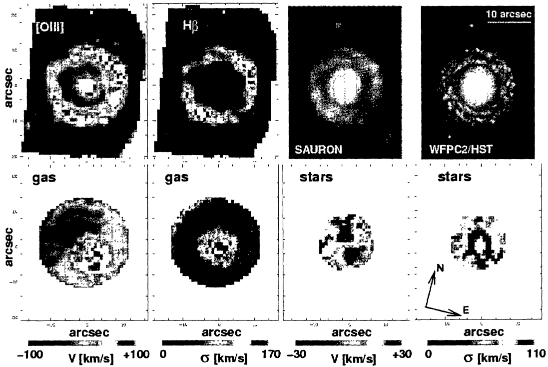
Figure 4. SAURON measurements of the stars and gas in NGC 7742, based on one pointing with seeing 1.5-2". The top row shows the emission-line intensity distributions of [OIII] and H\beta , followed by a reconstructed image composed of [OIII] and stellar continuum and a similar HST/WFPC2 image composed of F336W, F555W, and F814W exposures. The bottom row shows the derived gas velocity and velocity dispersion fields, followed by the stellar velocity and velocity dispersion.
