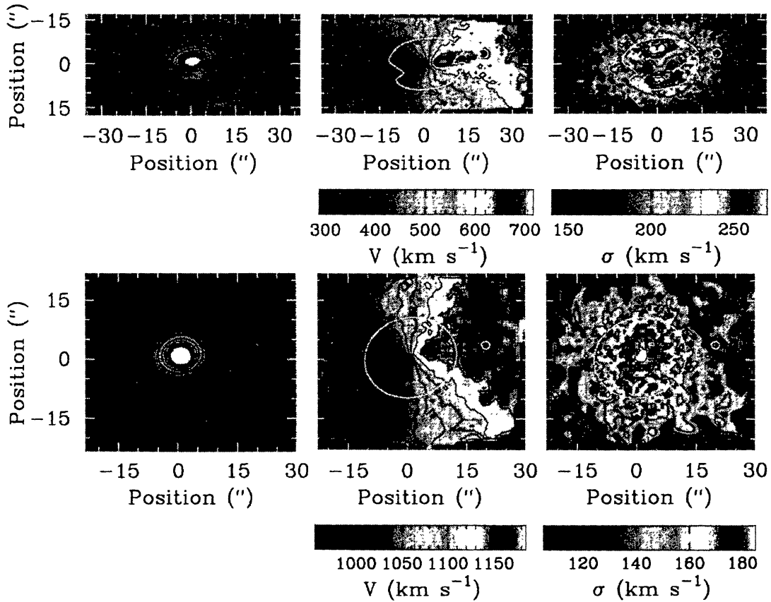
Figure 3. SAURON absorption-line measurements of the SB0 galaxies NGC 4526 and NGC 4459, both based on two partially overlapping pointings. Top row: Reconstructed total intensity, mean stellar velocity, and velocity dispersion fields of NGC 4526. Bottom row: Same for NGC 4459. Isophotes are overlaid on all fields as a reference.
