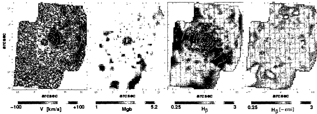
Figure 6. SAURON maps of NGC 5813, based on two partially overlapping pointings with seeing 1 - 2'' . From left to right: Stellar (mean) velocity field, Mg b map, raw H\beta map, and H\beta map corrected for emission. Isophotes are superposed on the first three images.
