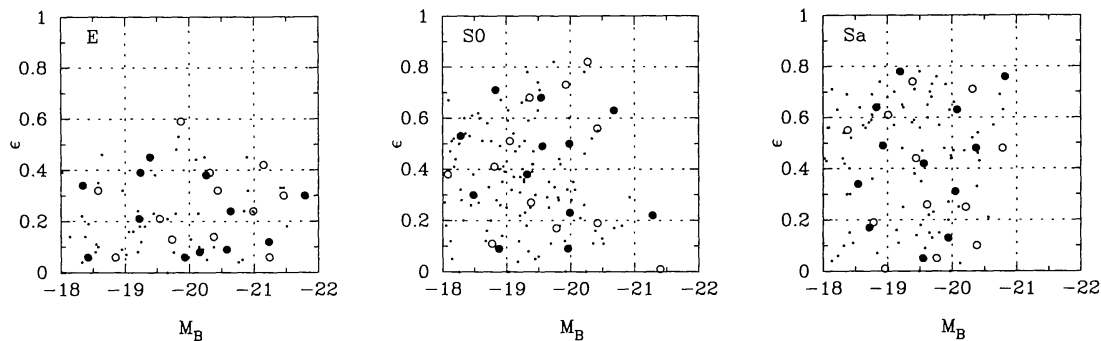
Figure 1. Distribution of E, S0, and Sa galaxies in the SAURON representative sample, in the planes of ellipticity \varepsilon versus absolute blue magnitude M_B . Open circles: field galaxies. Filled circles: cluster galaxies. Small dots: remaining galaxies of the complete sample.
